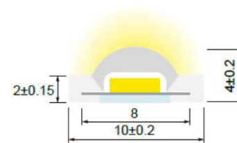
Cross section
