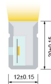
Unit: mm Cross section
