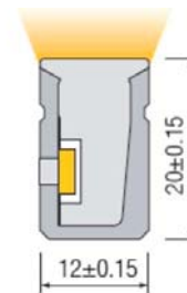
Unit: mm Cross section
