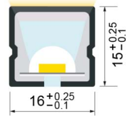
Unit: mm Cross section
